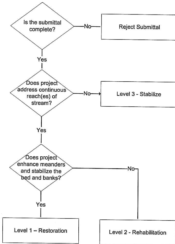
FIGURE 3 –Project Review Flow Chart
