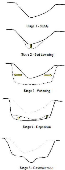
FIGURE 1 - Temporal process - changes occur at a point on a stream over time (Fischenich and Morrow, 2000)
